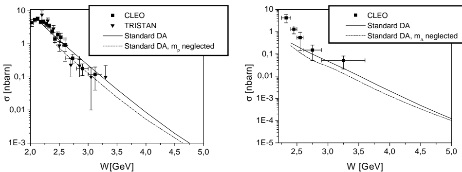
Fig. 1. Integrated \gamma\gamma \rightarrow p\bar{p} (left) and \gamma\gamma \rightarrow \Lambda\bar{\Lambda} (right) cross sections ( |\cos(\theta_{\text{cm}})| \leq 0.6 ) vs. W = \sqrt{s} . Solid (dash-dotted) line: predictions obtained with the standard parameterization of the diquark model (cf. Ref. 1) with (without) mass corrections. Data are taken from Refs. 7–9.
