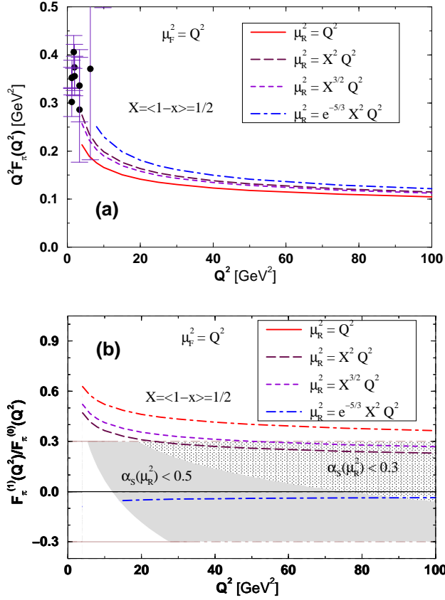
Fig. 1. (a) Leading-twist NLO QCD results for Q^2 F_\pi(Q^2) obtained using the \phi_{as}(x, \mu_F^2) distribution amplitude and the choices of \mu_R^2 given by Eqs. (6), (10–12), while \mu_F^2 = Q^2 and \langle \bar{x} \rangle = 0.5 . The experimental data are taken from Ref. 19. (b) The ratio F_\pi^{(1)}(Q^2)/F_\pi^{(0)}(Q^2) obtained using the same DA and the same choices for \mu_R^2 and \mu_F^2 scales as in Fig. 1a. The shaded area denotes the region of predictions which corresponds to F_\pi^{(1)}(Q^2)/F_\pi^{(0)}(Q^2) < 30\% , and \alpha_S(\mu_R^2) < 0.5 ( \alpha_S(\mu_R^2) < 0.3 ).
