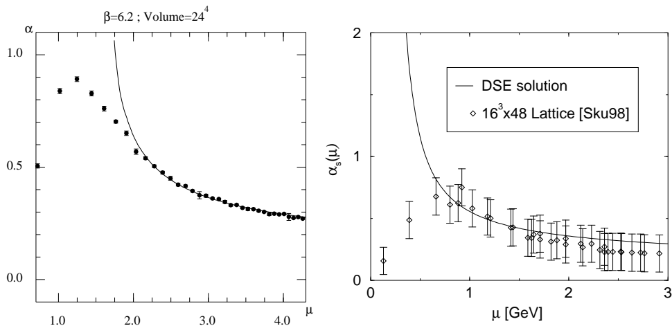
Fig. 1. Lattice results of the running coupling from the 3-gluon vertex (left, together with a 3-loop fit, Fig. 1 of Ref. 21), and from the quark-gluon vertex for \beta = 6.0 on a 16^3 \times 48 lattice (right, c.f. Fig. 2 of Ref. 22).
