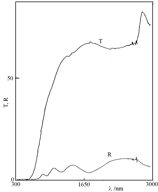
Fig. 3. Transmission, T and reflection, R , spectrum of a typical \text{Bi}_2\text{S}_3 thin film ( d \approx 590 nm).
