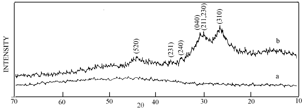
Fig. 1. X-ray diffraction patterns of chemically deposited \text{Bi}_2\text{S}_3 films: a) as deposited, b) annealed at 523 K for 35 min.
