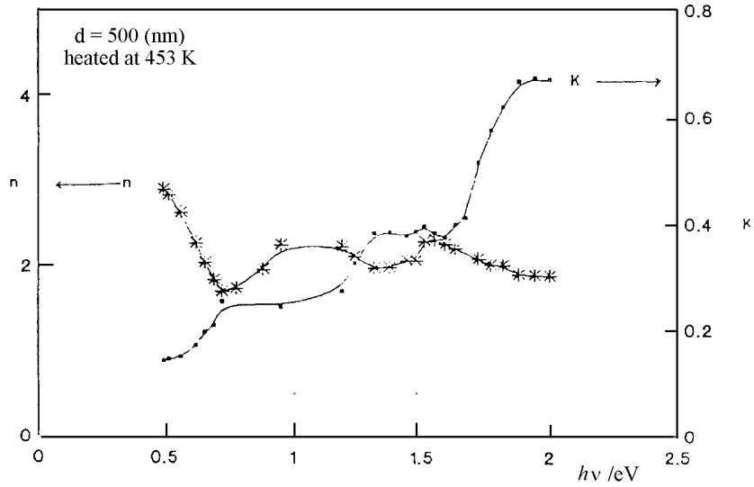
Fig. 8. Variation of the optical constants ( n, k ) with photon energy ( h\nu ) - thermally deposited film ( d \approx 500 nm heated at 453 K).
