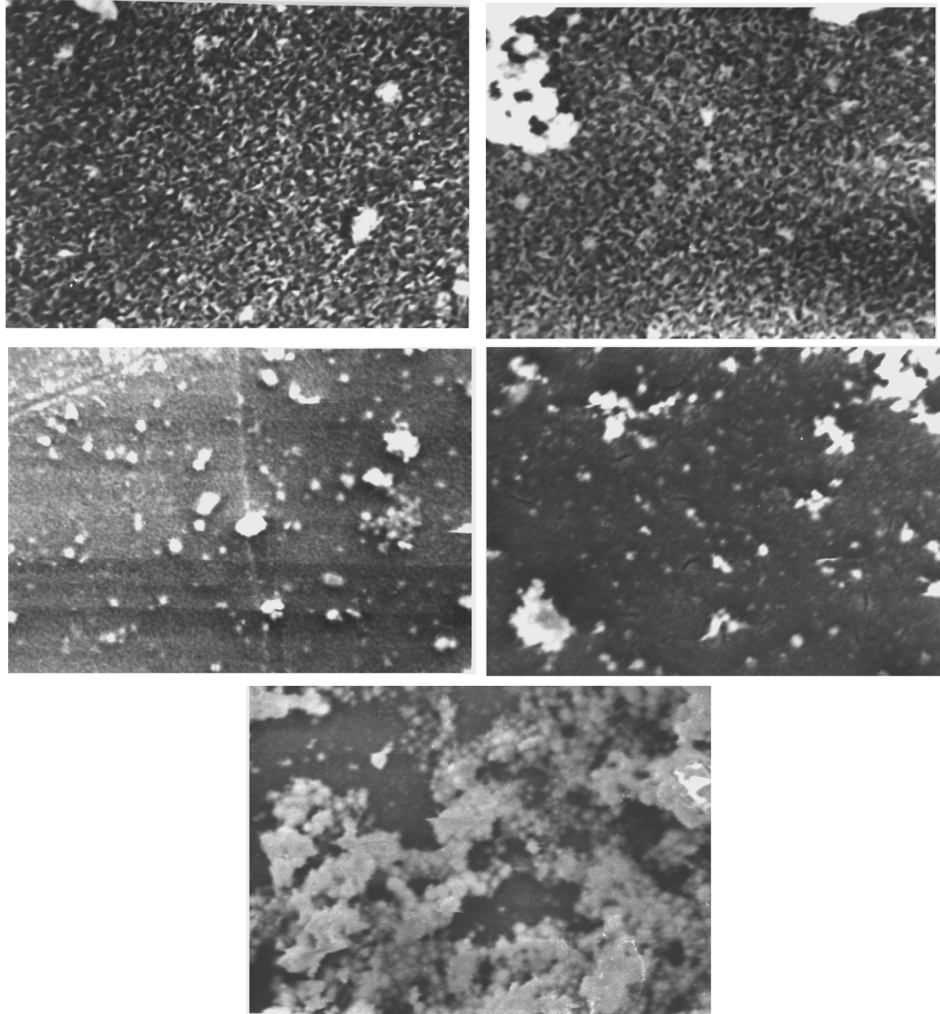
Fig. 2. Scanning electron micrograph of non-heated and heated chemically deposited Bi 2 S 3 films, each of a thickness d \approx 860 nm: a) non heated, 10 500 \times , b) heated at 523 K for 10 min., 10 500 \times , c) heated at 523 K for 35 min., 6000 \times , d) heated at 573 K for 10 min., 6000 \times , and e) heated at 573 K for 35 min., 6000 \times .
