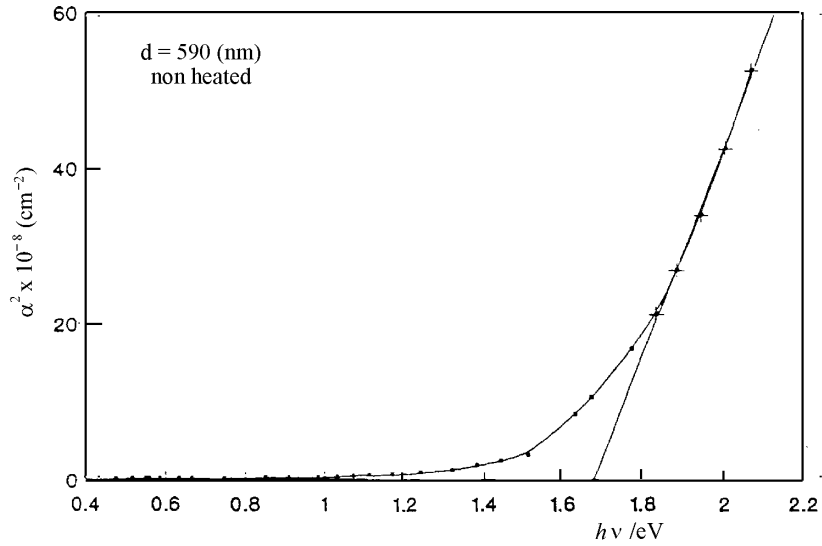
Fig. 7. Variation of \alpha^2 vs. h\nu ( d \approx 590 nm).
