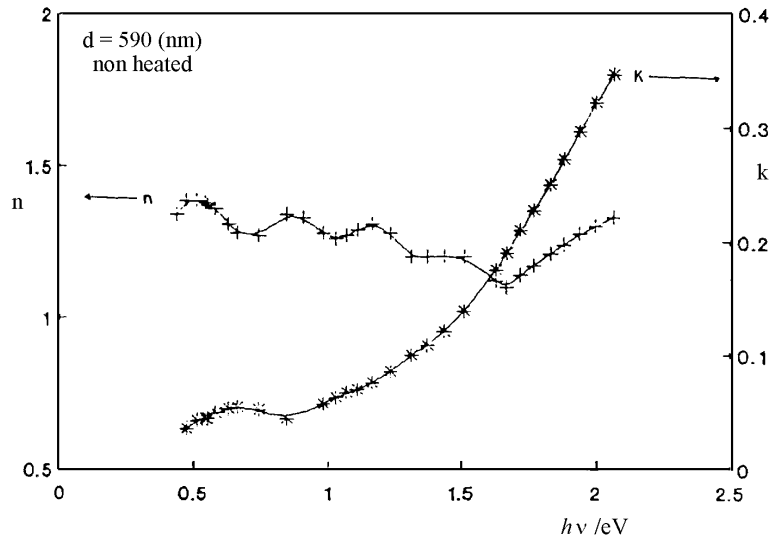
Fig. 4. Variation of the optical constants ( n, k ) with photon energy ( h\nu ) ( d \approx 590 nm).
