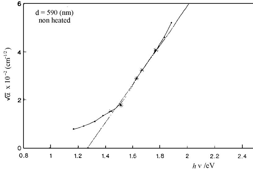
Fig. 6. Variation of \sqrt{\alpha} vs. h\nu ( d \approx 590 nm).
