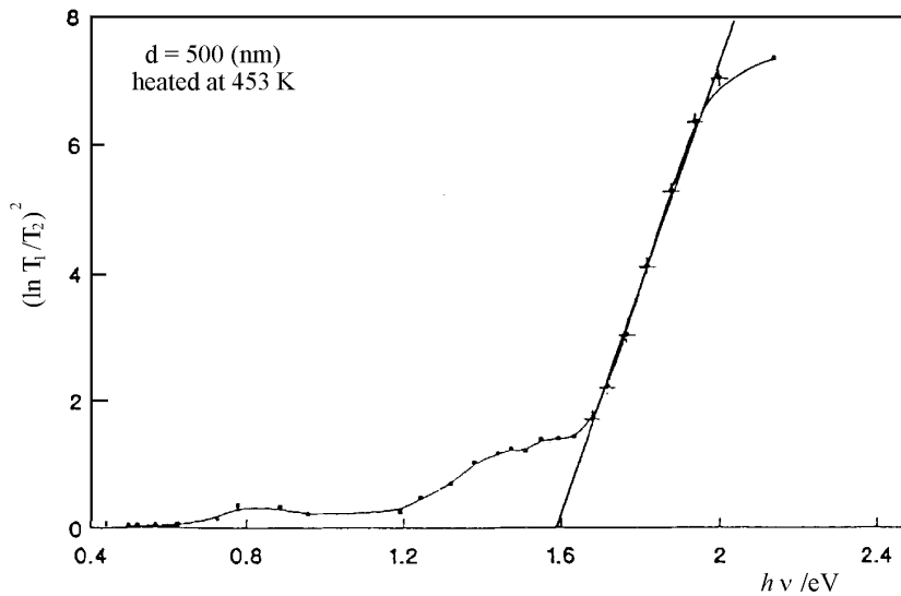
Fig. 9. (\ln T_1/T_2)^2 vs. h\nu for thermally deposited \text{Bi}_2\text{S}_3 film ( d \approx 500 nm).
