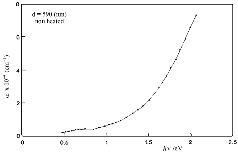
Fig. 5. Variation of optical absorption coefficient ( \alpha ) with photon energy ( h\nu ) ( d \approx 590 nm).
