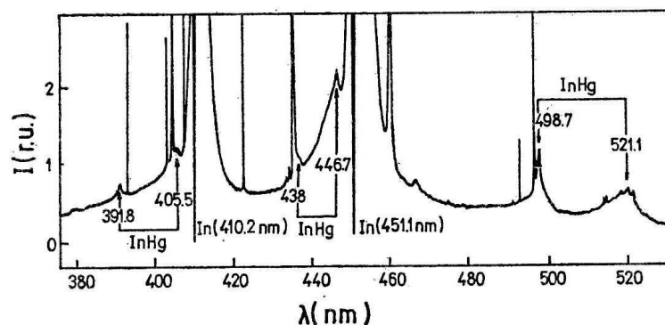
Fig. 4. The spectrum of InI-Hg-Ar discharge lamp in the spectral region from 380 to 530 nm, recorded in current reversal mode.
