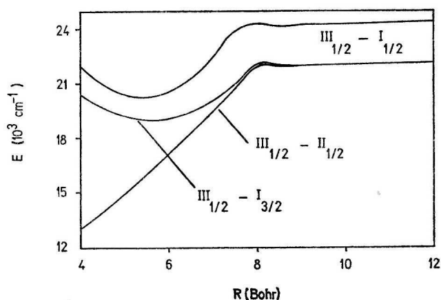
Fig. 7. The sketch of the difference potentials for the III_{1/2}-I_{1/2} , III_{1/2}-I_{3/2} and III_{1/2}-II_{1/2} , transitions.
