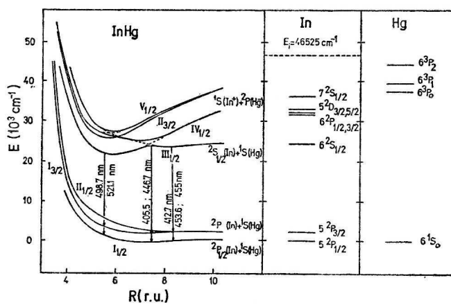
Fig. 6. Qualitative picture of the potential energy curves for InHg excimer, together with the atomic energy levels of In and Hg.
