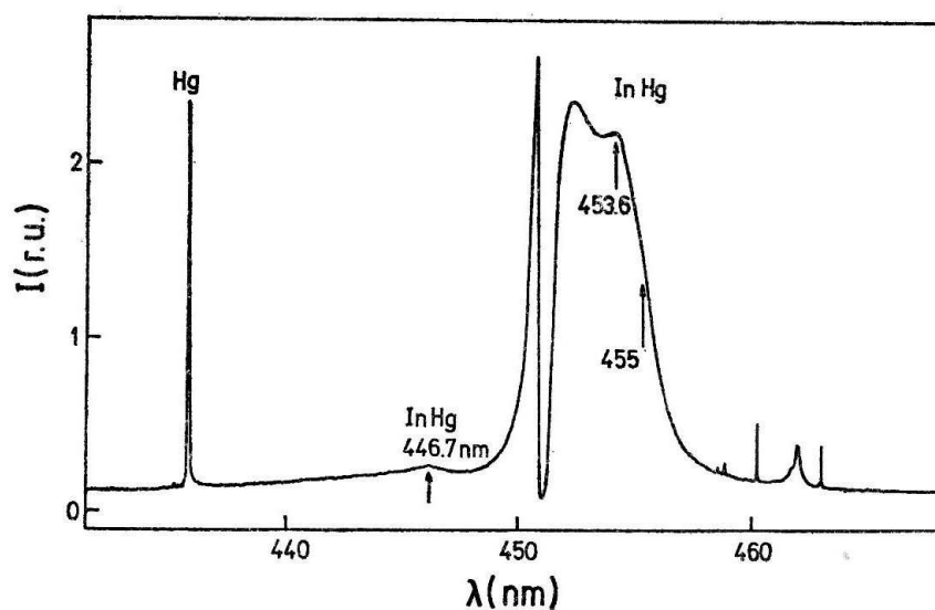
Fig. 2. The region of In resonance line at 451.1 nm, with three satellites at 453.6, 455 and 446.7 nm.
