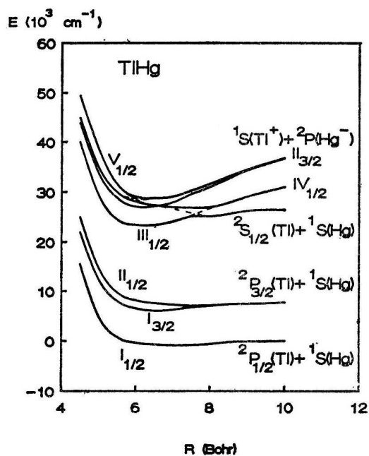
Fig. 5. The ab initio potential energy curves for TIHg excimer calculated by Calvert-Celestino and Emler (Ref. 12).
