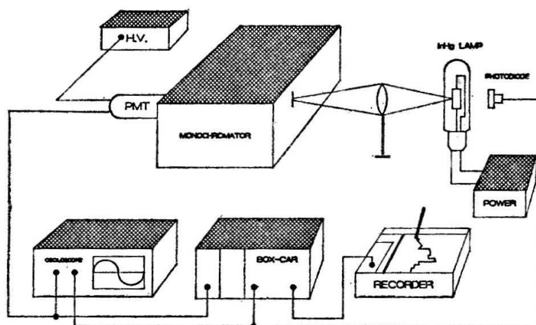
Fig. 1. Experimental arrangement.
