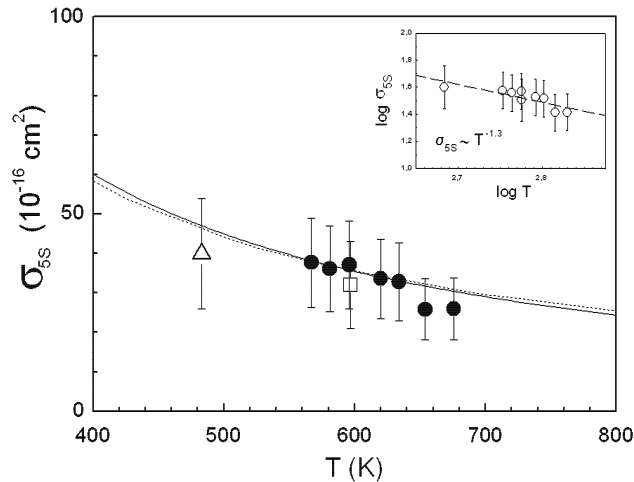
Fig. 2. The cross section \sigma_{5S} for the energy pooling process \text{Na}(3P) + \text{Na}(3P) \rightarrow \text{Na}(5S) + \text{Na}(3S) , as a function of temperature. Experimental results: triangle - Allegrini et al. [11], square - Huennekens and Gallagher [10], full dots - present work. Theoretical result: dotted line - recent theoretical calculation of Yurova [17]; the curve displayed is obtained as a weighted average of the (J, J') - selective cross sections (data are digitised from the figures in the original paper) given in [17] to enable correct comparison with the present experiment in which the fine-structure levels of the initial 3P state were populated in the statistical ratio. The determination of the \sigma_{5S} temperature dependence is illustrated in the inset. All available experimental data are included in the analysis, yielding \sigma_{5S} \propto T^{-1.3} dependence, which is indicated with full line in the picture.
